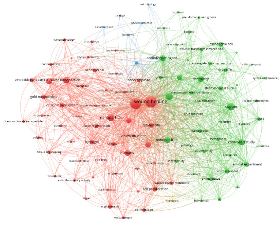
Fig. 3. Thematic distribution of the analyzed topic using the tools of bibliometric analysis VOSviewer
